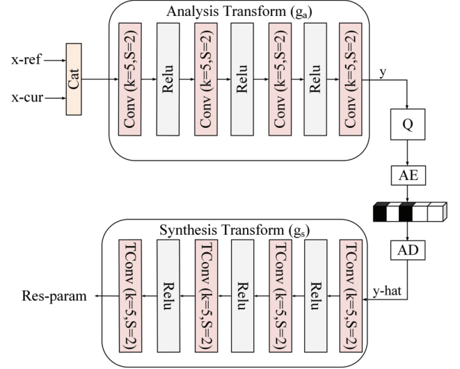
Fig. 2. Structure of the spectral residual compression network. AE stands for Arithmetic Encoder, AD stands for Arithmetic Decoder, and Q represents the Quantizer.
