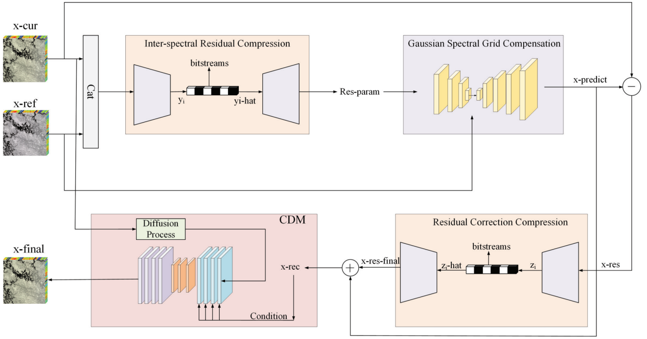
Fig. 1. Overall BRC-CDM network. Here, y_i denotes the latent representation extracted by the interband residual compression network. \hat{y}_i represents the reconstructed latent feature obtained by decoding the quantized bitstream using an AD, which serves as the input to the decoder module. Similarly, z_i denotes the latent representation produced by the residual correction compression network, and \hat{z}_i refers to its decoded version, also recovered via arithmetic decoding and fed into the corresponding decoder. The spectral residual compression network encodes the residuals between the current and reference bands, producing a three-channel residual map. The SGGC module utilizes spatial-spectral residuals to adjust the reference band and predict the current band. The residual correction network compresses the difference. The compressed representation of the current band serves as a latent condition to guide the sampling trajectory in the CDM.
