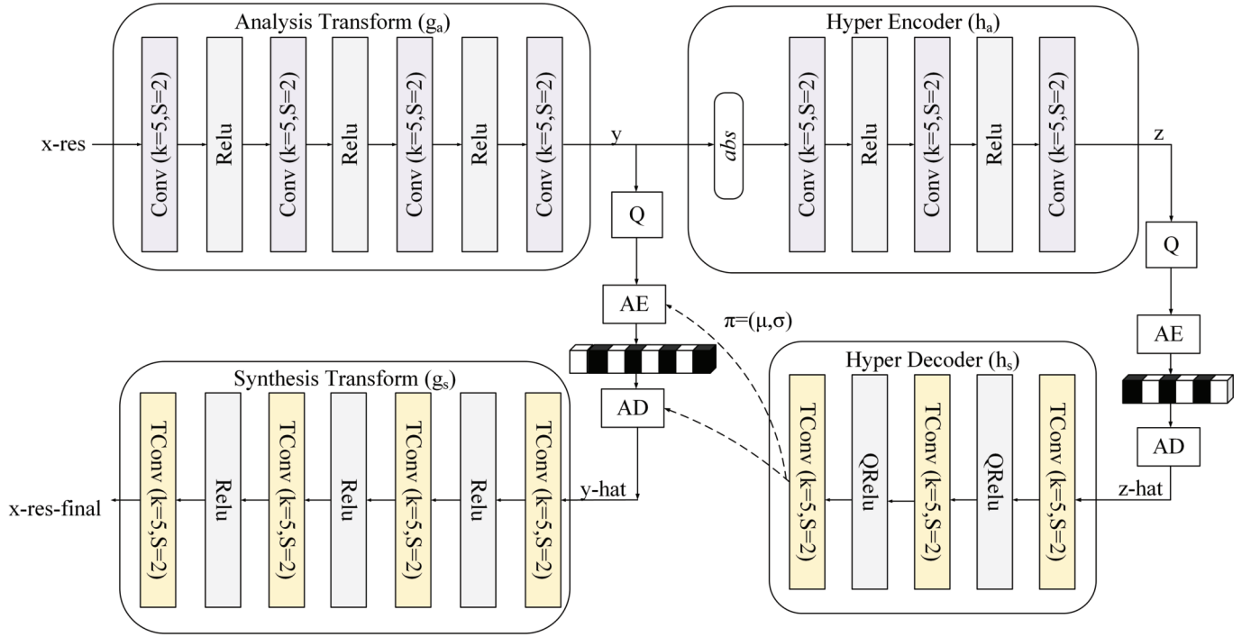
Fig. 3. Structure of the residual correction compression network.
