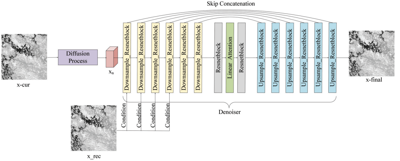
Fig. 4. Structure of the CDM.
