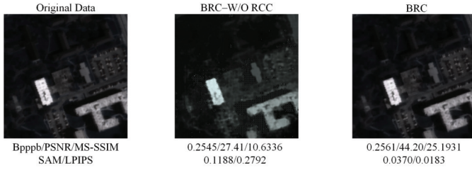
Fig. 8. Visualization of Washington dc dataset on ablation study.
